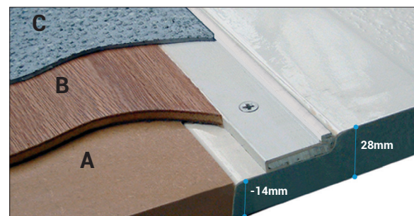
A - Floorboard or concrete flooring B - 1/4 Plywood C - 2mm vinyl sheet flooring
