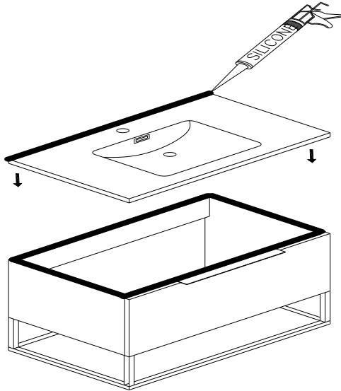
Silicone Sealant
