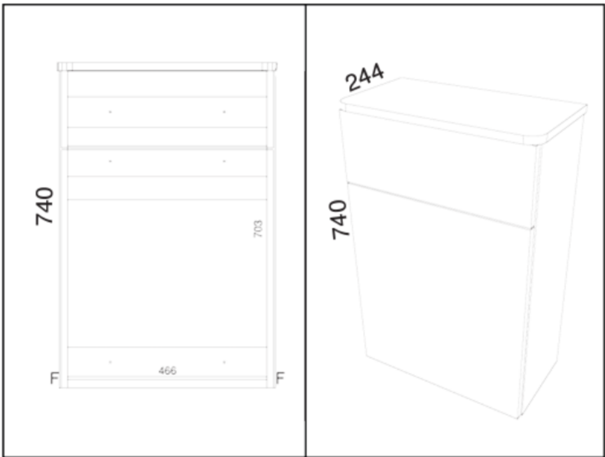
Technical drawing
